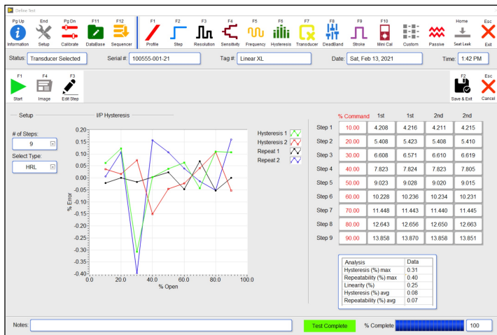
Hysteresis
