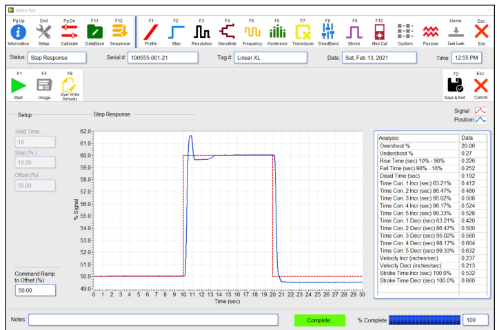
Step Response
